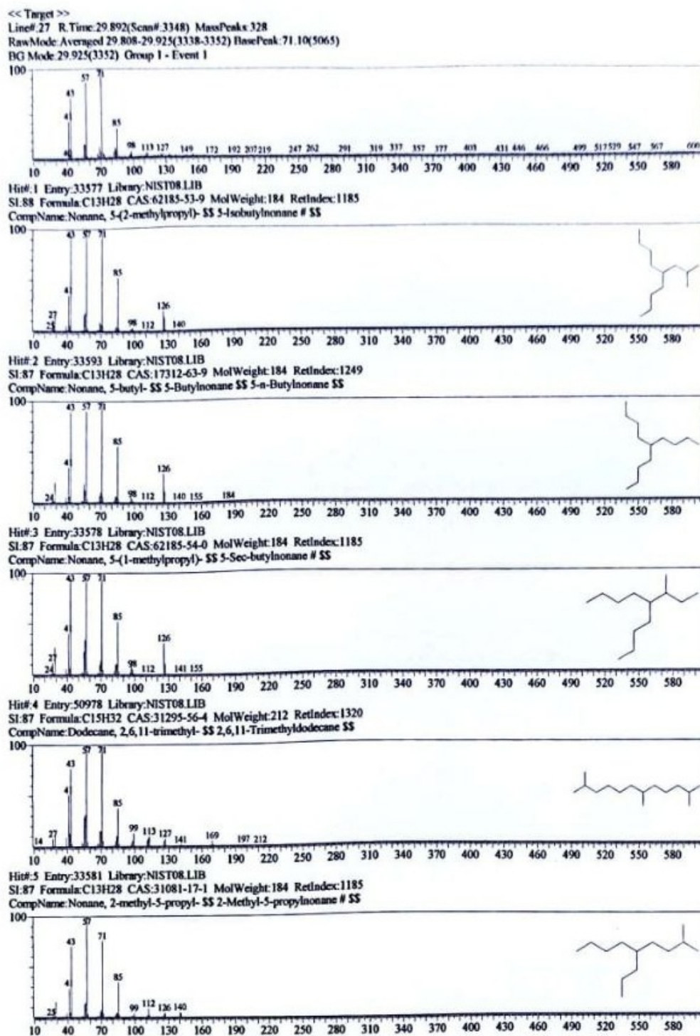
Figure 3. GC–MS mass-spectral library-search output, panel 1 of 27; candidate matches are tentative and not confirmed compound identities.
