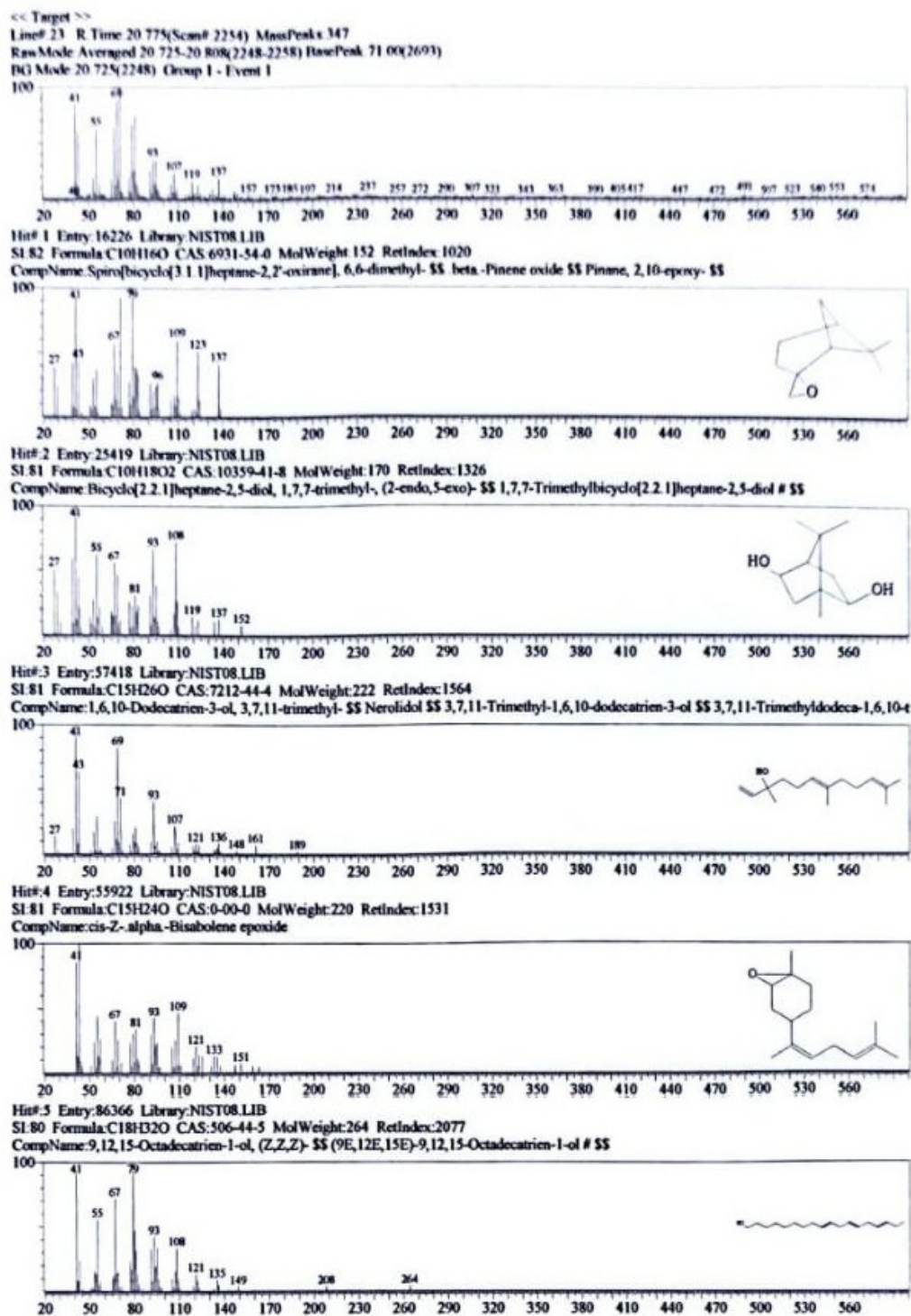
Figure 4. GC-MS mass-spectral library-search output, panel 2 of 27; candidate matches are tentative and not confirmed compound identities.
