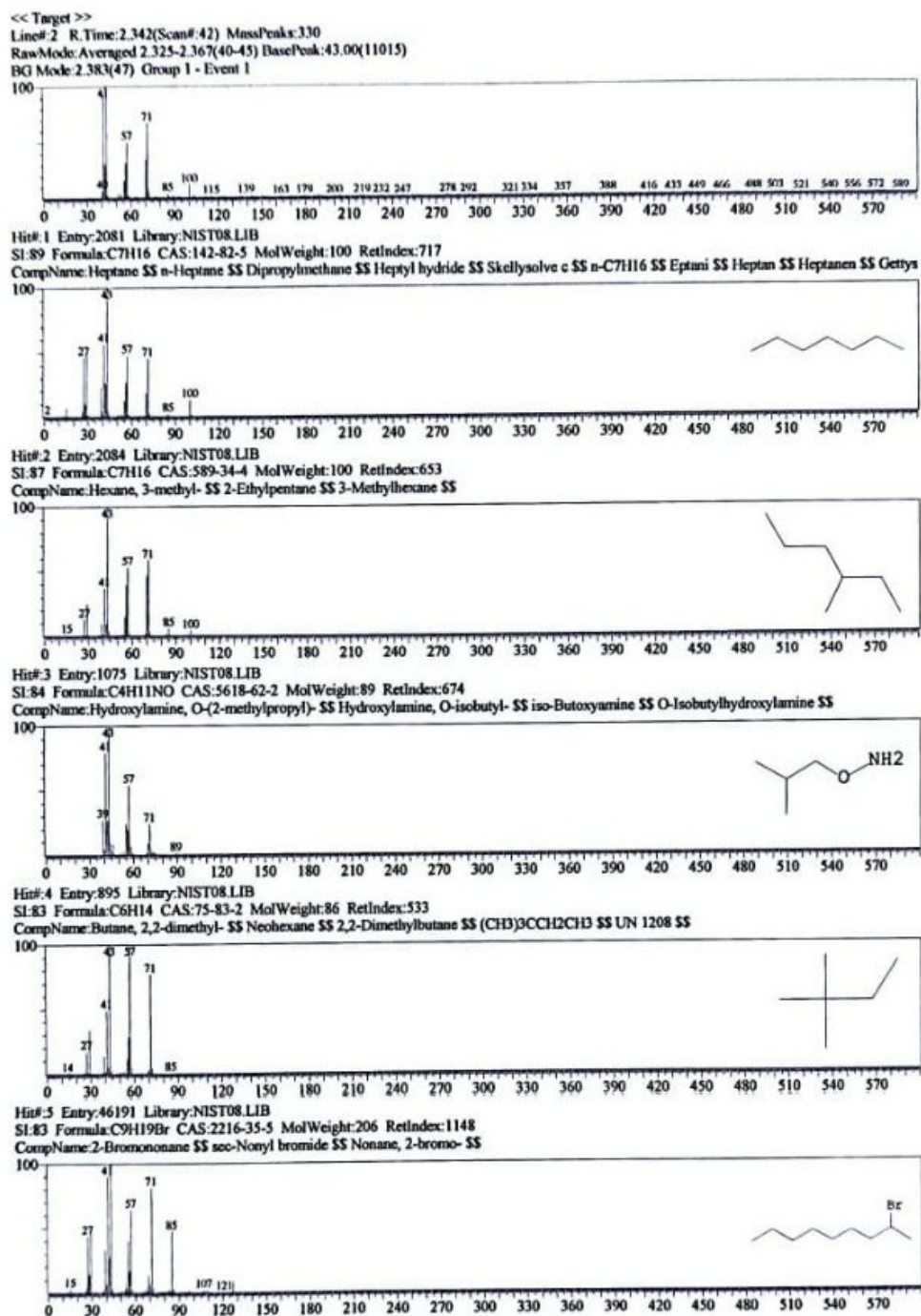
Figure 24. GC-MS mass-spectral library-search output, panel 22 of 27; candidate matches are tentative and not confirmed compound identities.
