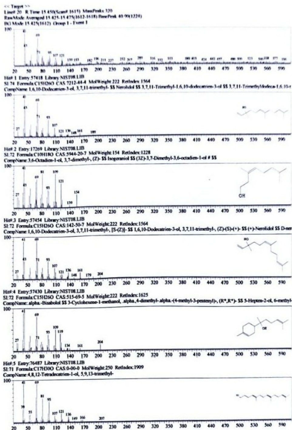
Figure 15. GC-MS mass-spectral library-search output, panel 13 of 27; candidate matches are tentative and not confirmed compound identities.
