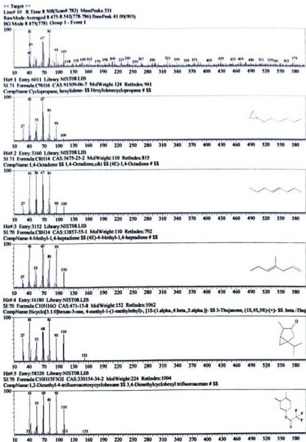
Figure 26. GC-MS mass-spectral library-search output, panel 24 of 27; candidate matches are tentative and not confirmed compound identities.
