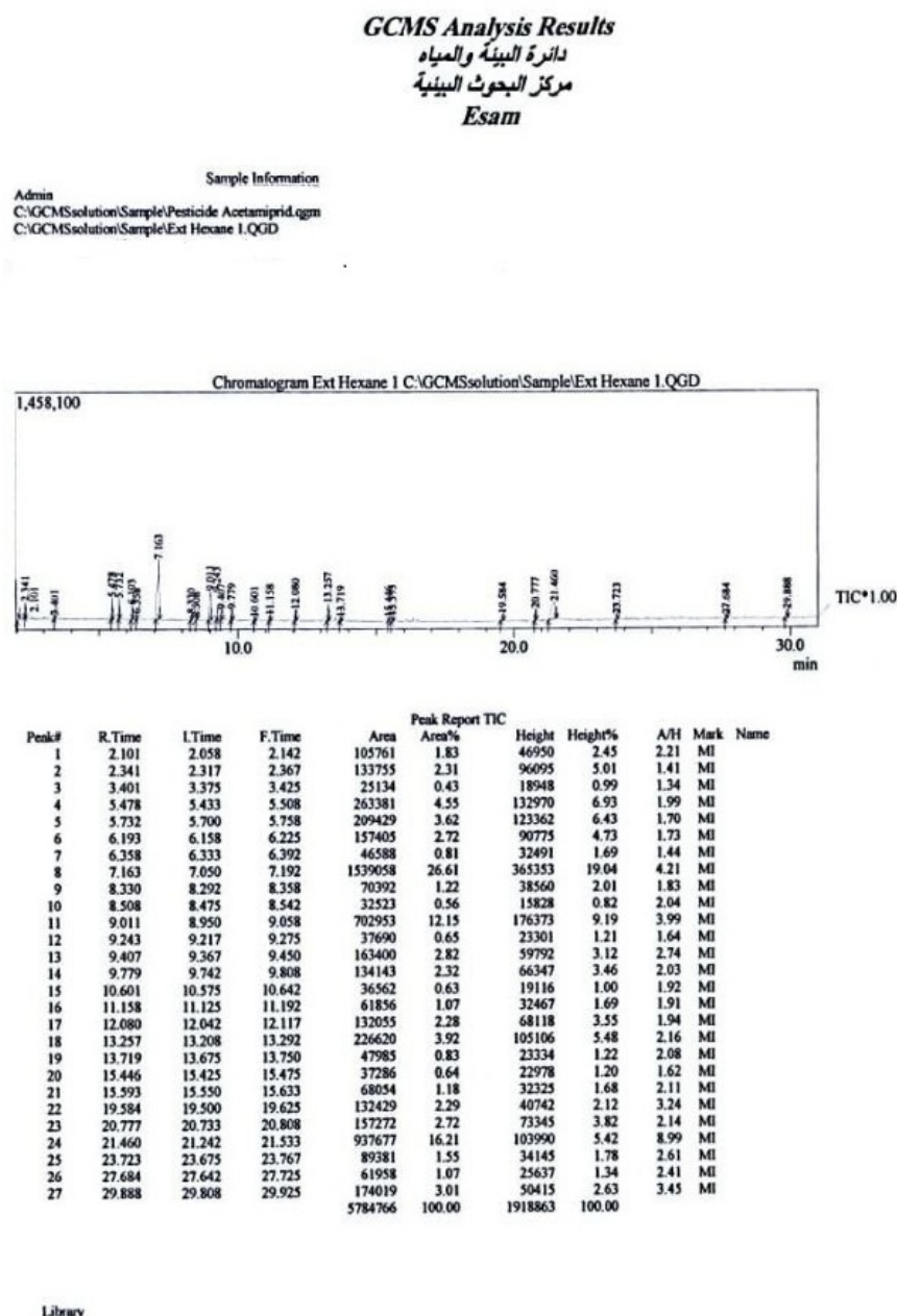
Figure 2. GC-MS total-ion chromatogram and peak report for the extract, reproduced from the supplied analytical output; solvent annotation requires verification.
