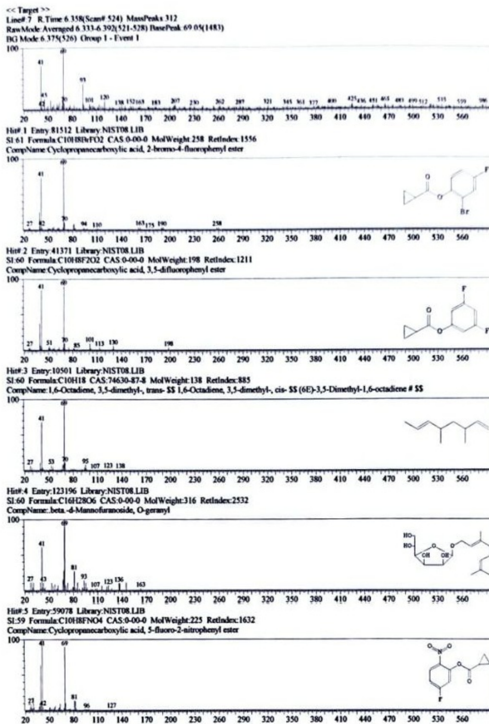
Figure 19. GC-MS mass-spectral library-search output, panel 17 of 27; candidate matches are tentative and not confirmed compound identities.
