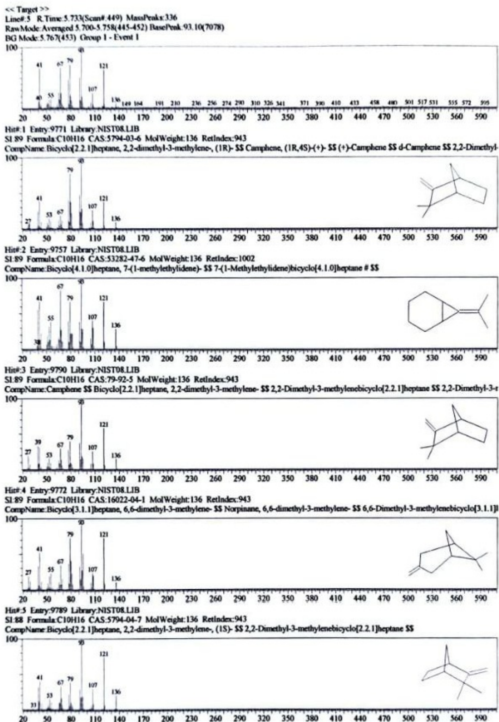
Figure 22. GC-MS mass-spectral library-search output, panel 20 of 27; candidate matches are tentative and not confirmed compound identities.
