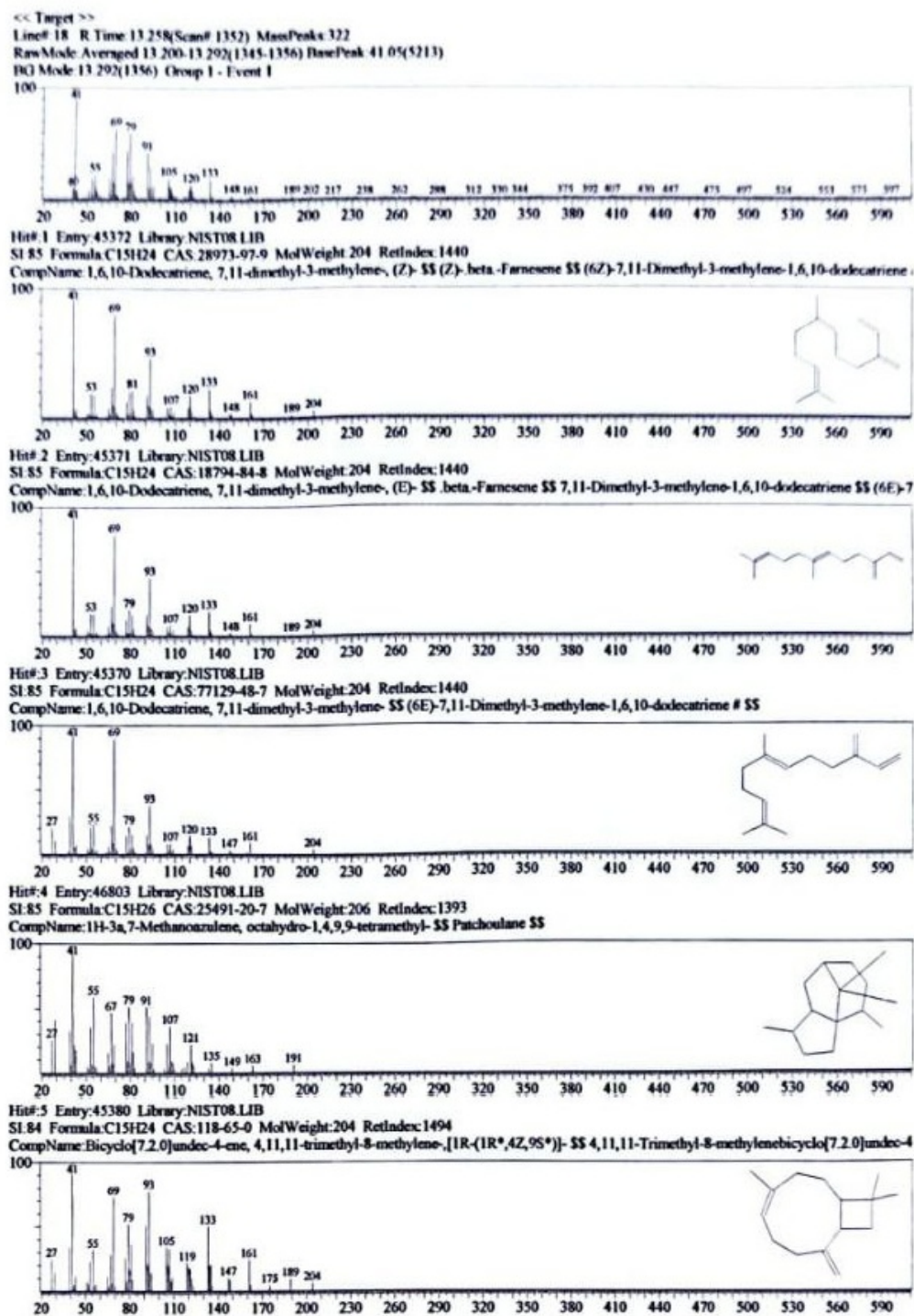
Figure 11. GC-MS mass-spectral library-search output, panel 9 of 27; candidate matches are tentative and not confirmed compound identities.
