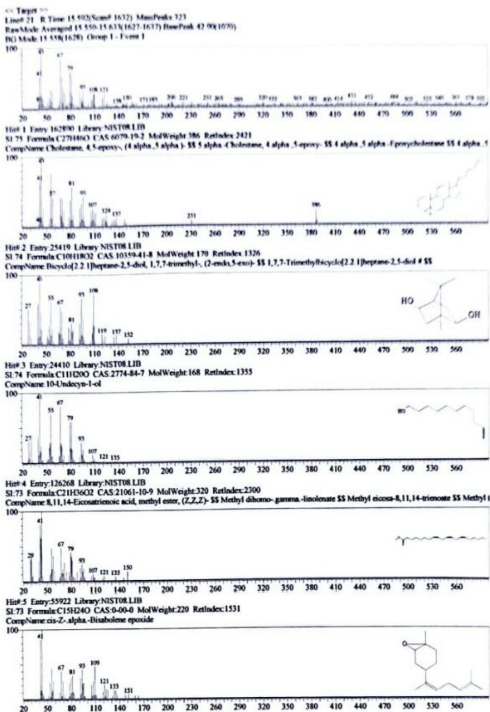
Figure 9. GC-MS mass-spectral library-search output, panel 7 of 27; candidate matches are tentative and not confirmed compound identities.
