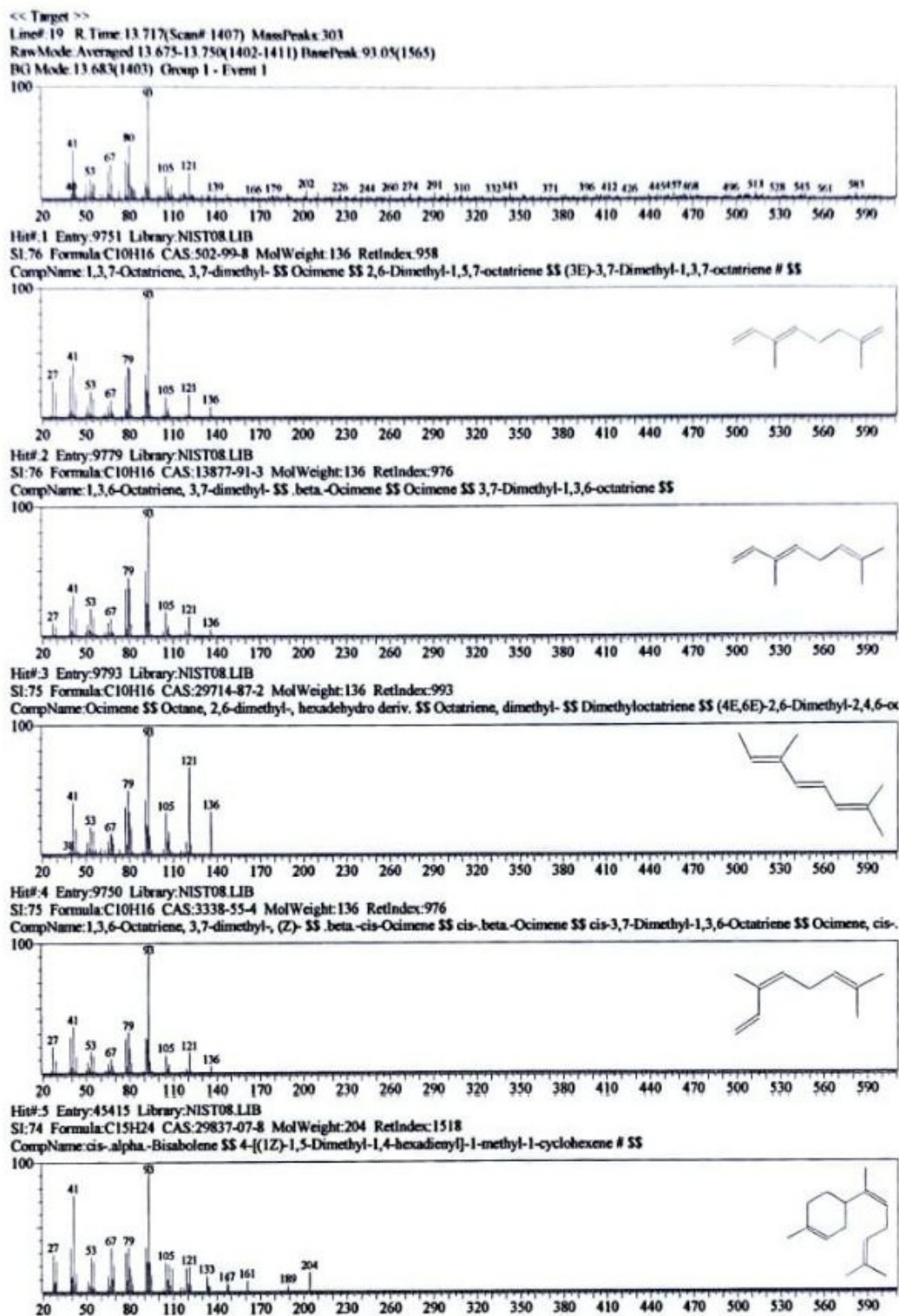
Figure 10. GC-MS mass-spectral library-search output, panel 8 of 27; candidate matches are tentative and not confirmed compound identities.
