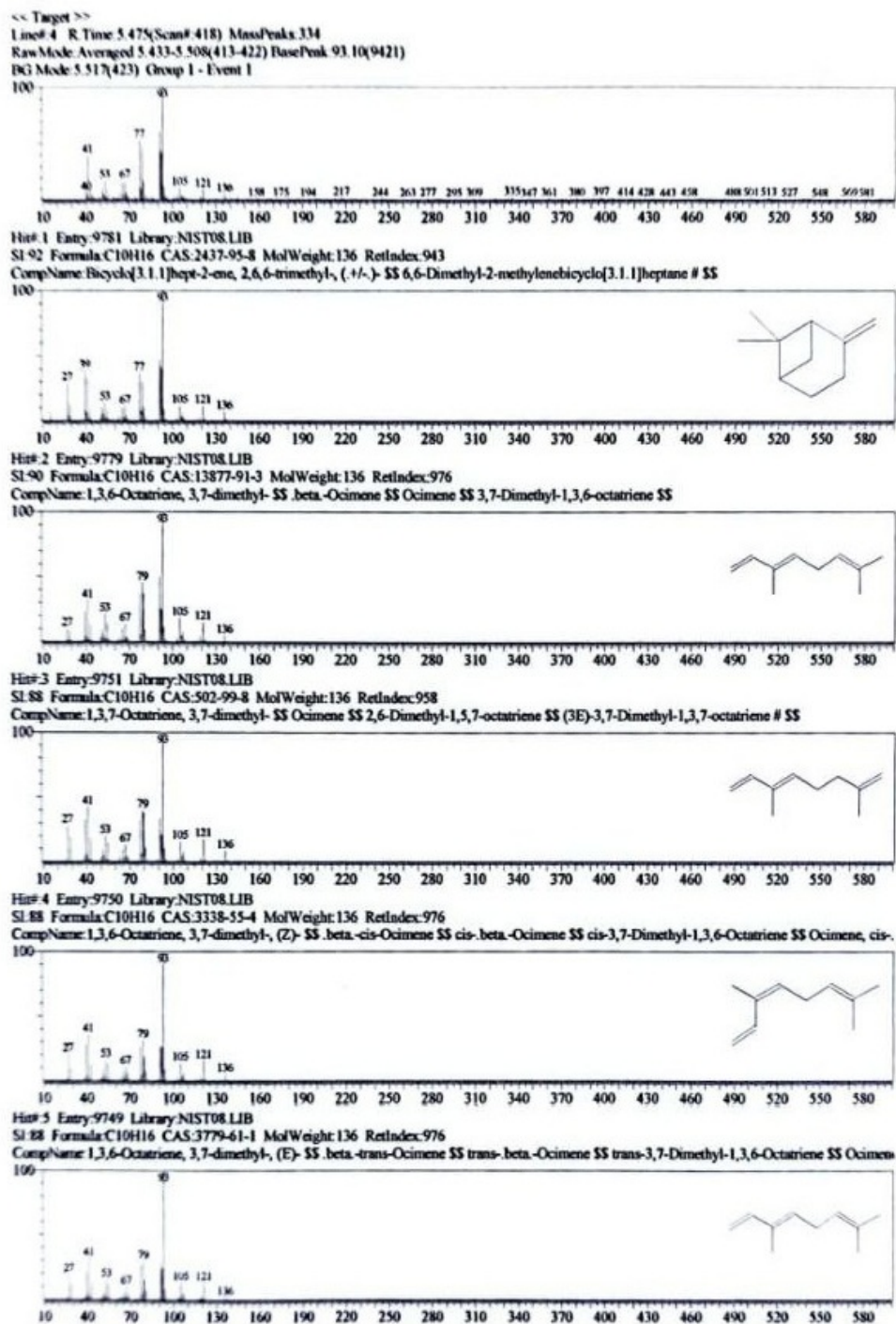
Figure 21. GC-MS mass-spectral library-search output, panel 19 of 27; candidate matches are tentative and not confirmed compound identities.
