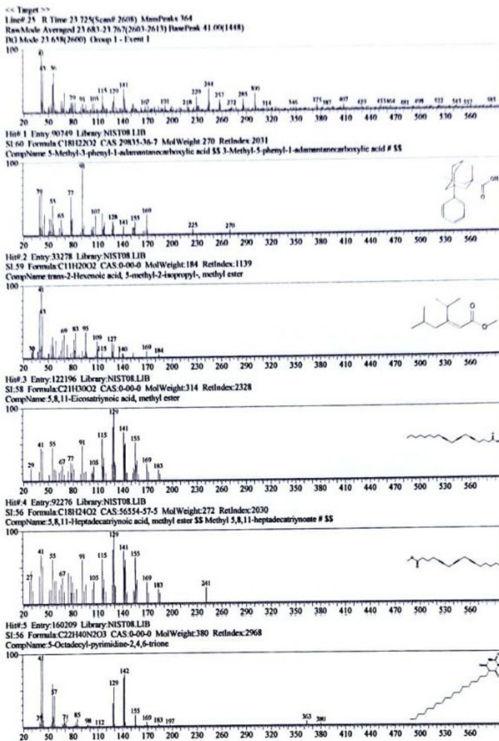
Figure 6. GC-MS mass-spectral library-search output, panel 4 of 27; candidate matches are tentative and not confirmed compound identities.
