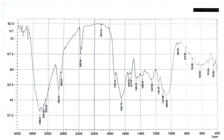
Figure 1. Infrared spectrum of the sage sample, reproduced from the author-supplied PDF. Functional-group assignments remain provisional.
