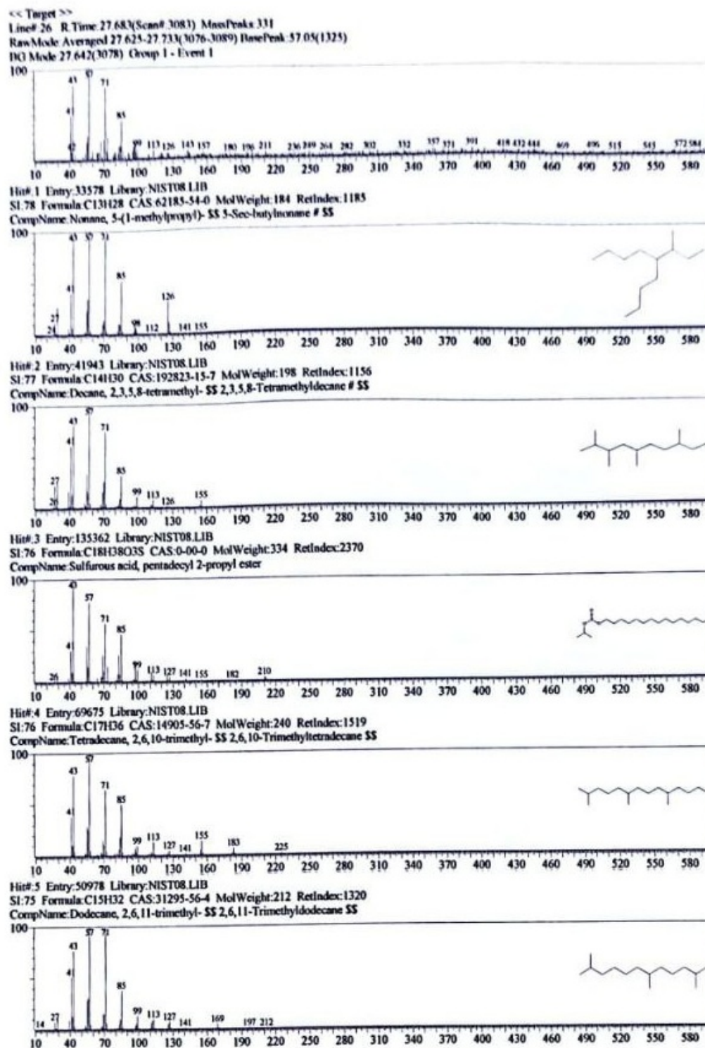
Figure 7. GC-MS mass-spectral library-search output, panel 5 of 27; candidate matches are tentative and not confirmed compound identities.
