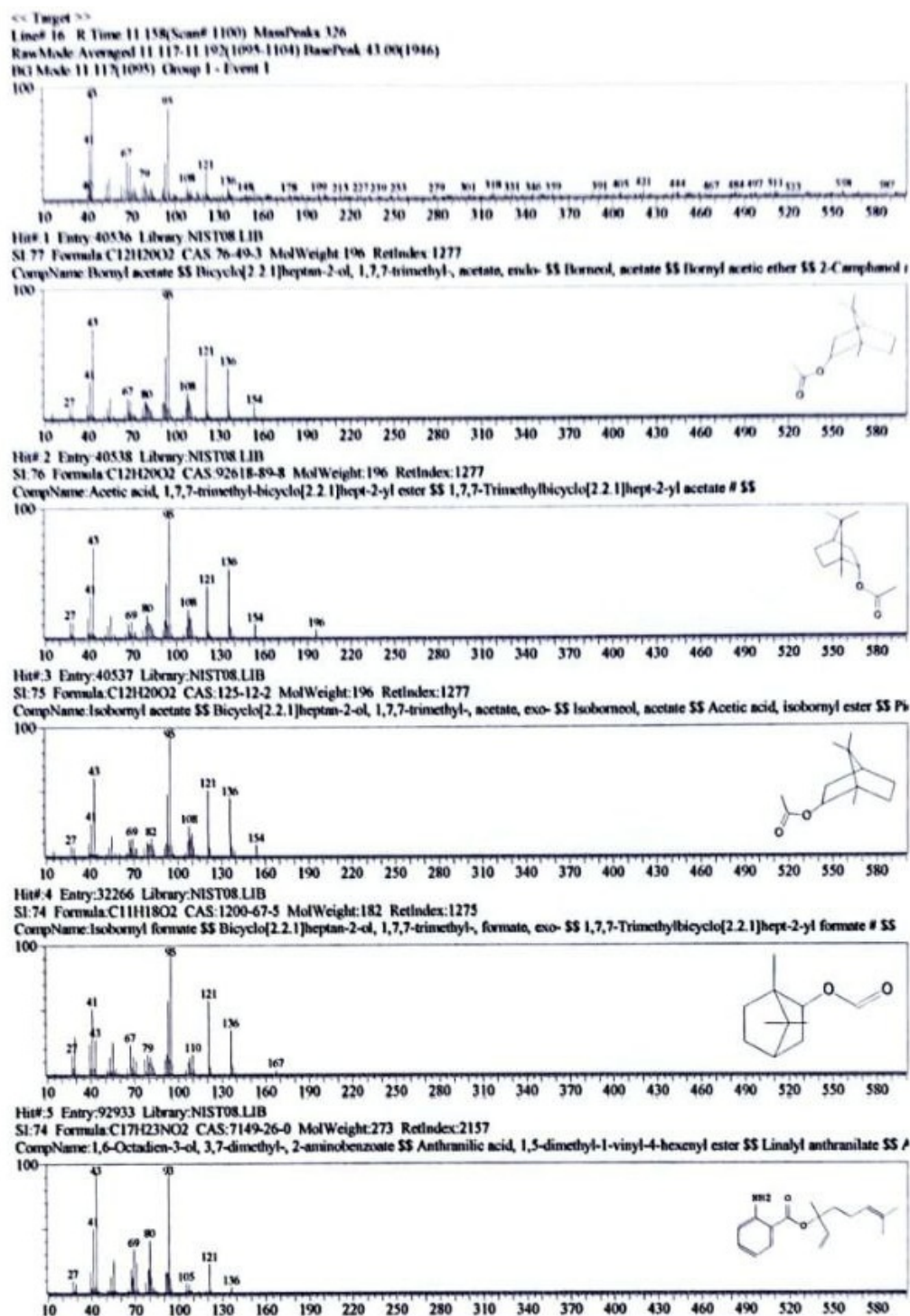
Figure 13. GC-MS mass-spectral library-search output, panel 11 of 27; candidate matches are tentative and not confirmed compound identities.
