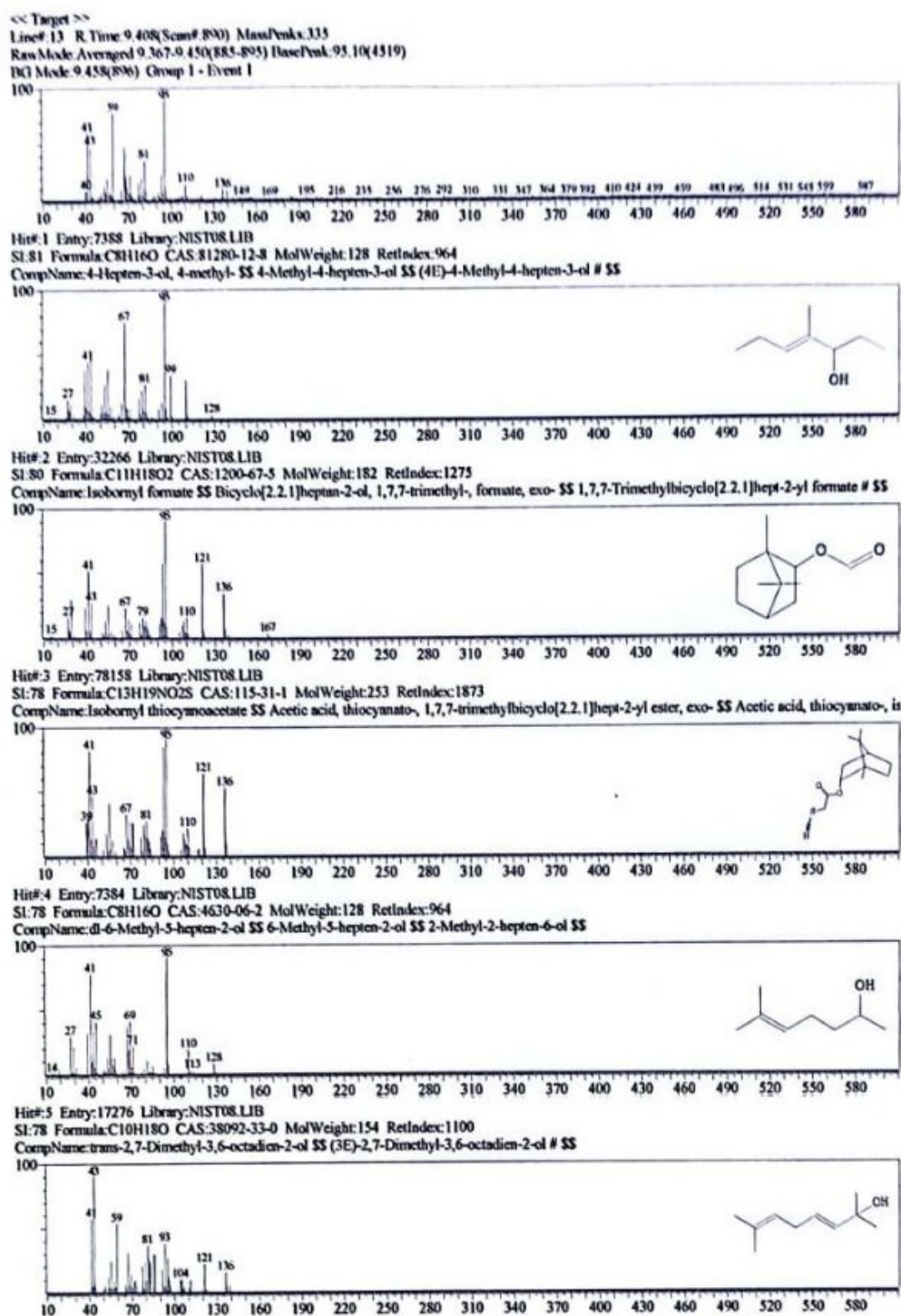
Figure 29. GC-MS mass-spectral library-search output, panel 27 of 27; candidate matches are tentative and not confirmed compound identities.
