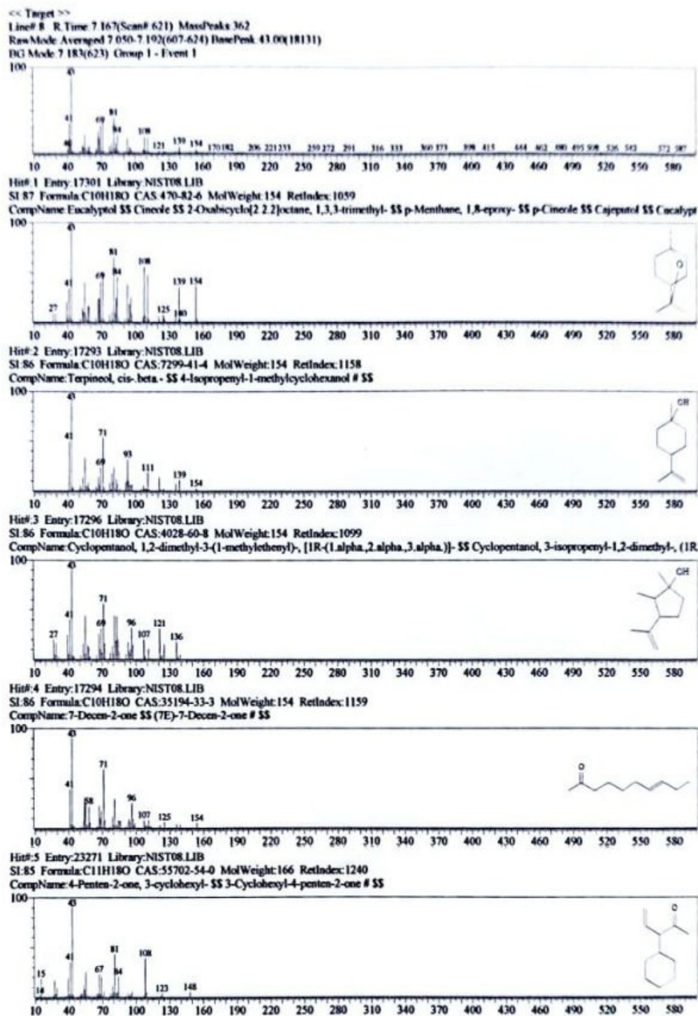
Figure 18. GC-MS mass-spectral library-search output, panel 16 of 27; candidate matches are tentative and not confirmed compound identities.
