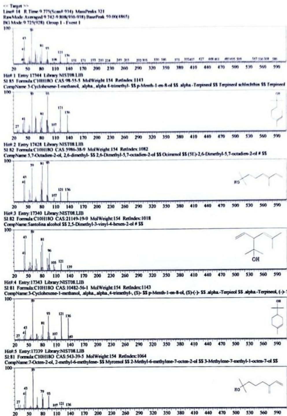
Figure 16. GC-MS mass-spectral library-search output, panel 14 of 27; candidate matches are tentative and not confirmed compound identities.
