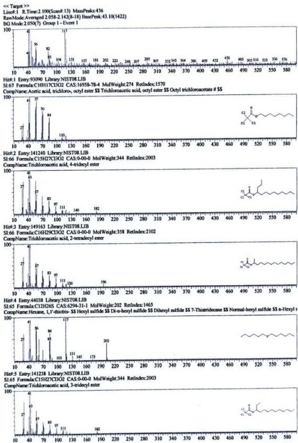
Figure 25. GC-MS mass-spectral library-search output, panel 23 of 27; candidate matches are tentative and not confirmed compound identities.
