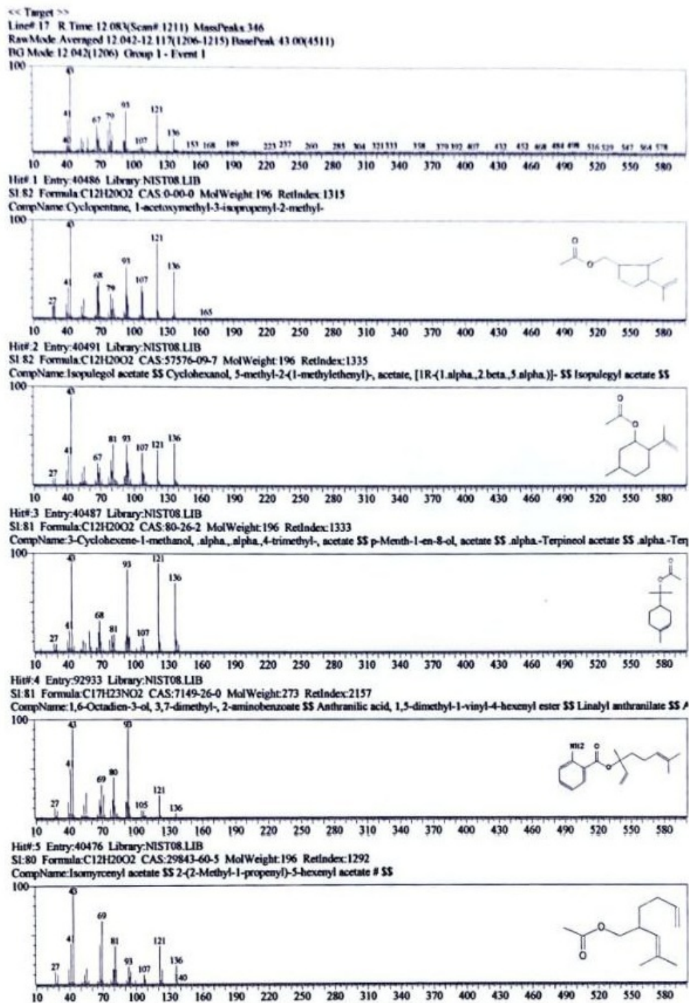
Figure 14. GC-MS mass-spectral library-search output, panel 12 of 27; candidate matches are tentative and not confirmed compound identities.
