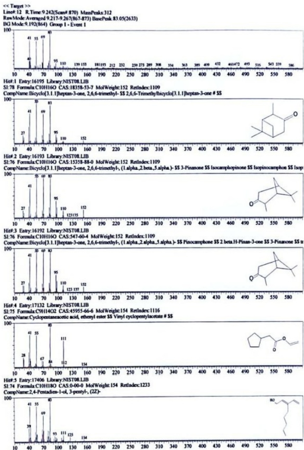
Figure 28. GC-MS mass-spectral library-search output, panel 26 of 27; candidate matches are tentative and not confirmed compound identities.
