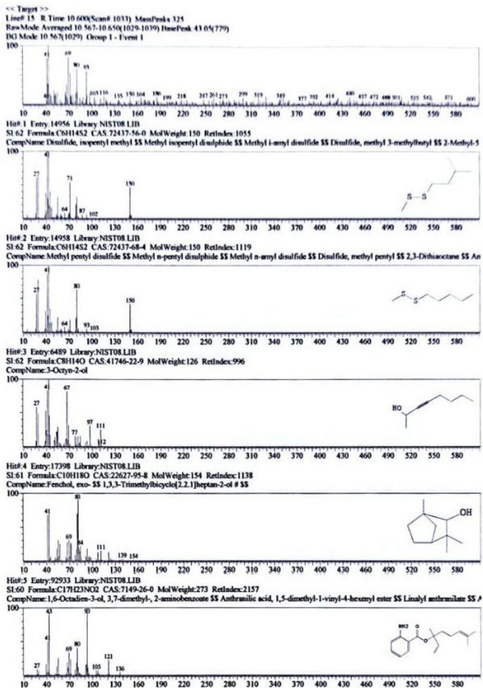
Figure 12. GC-MS mass-spectral library-search output, panel 10 of 27; candidate matches are tentative and not confirmed compound identities.
