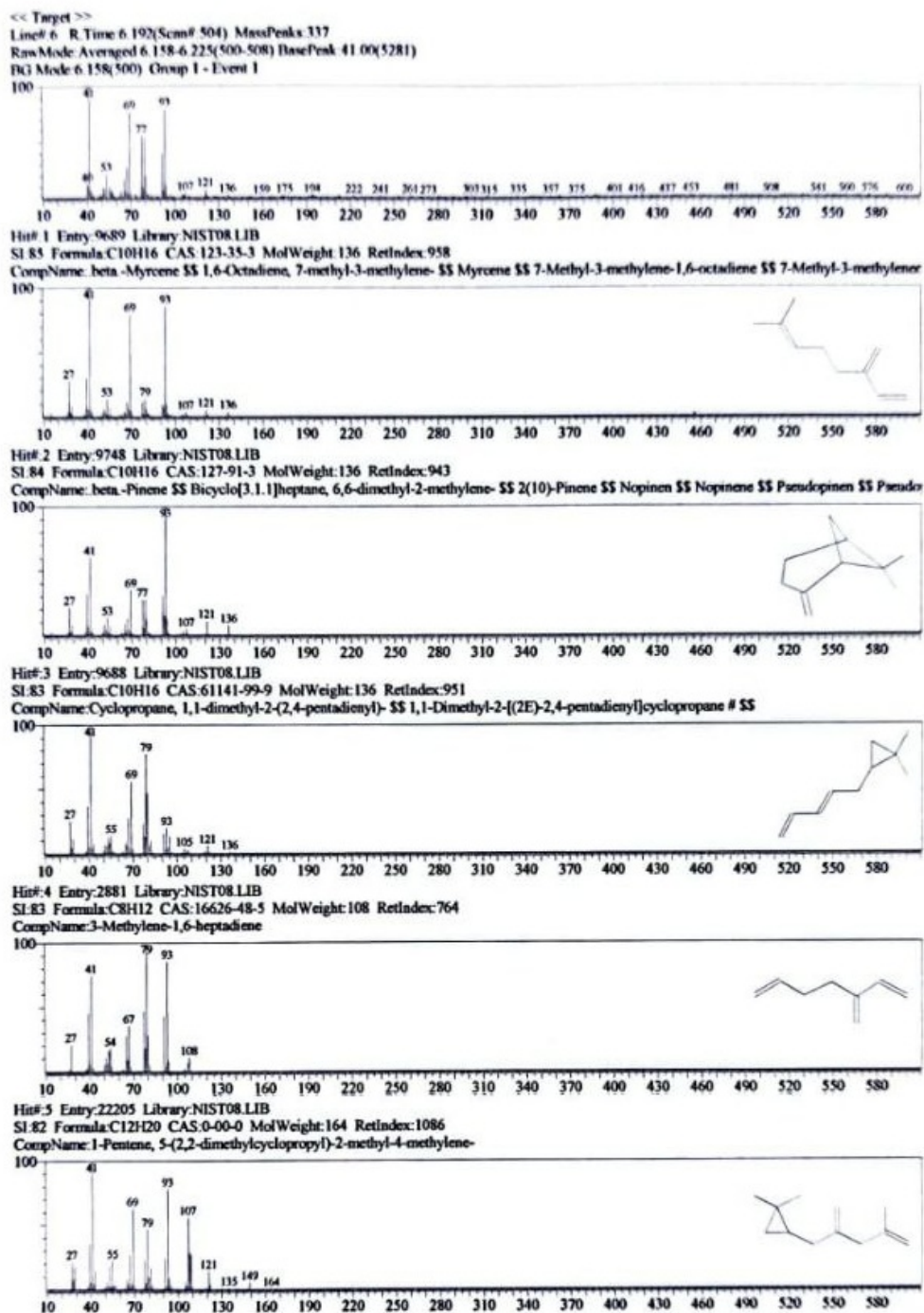
Figure 23. GC-MS mass-spectral library-search output, panel 21 of 27; candidate matches are tentative and not confirmed compound identities.
