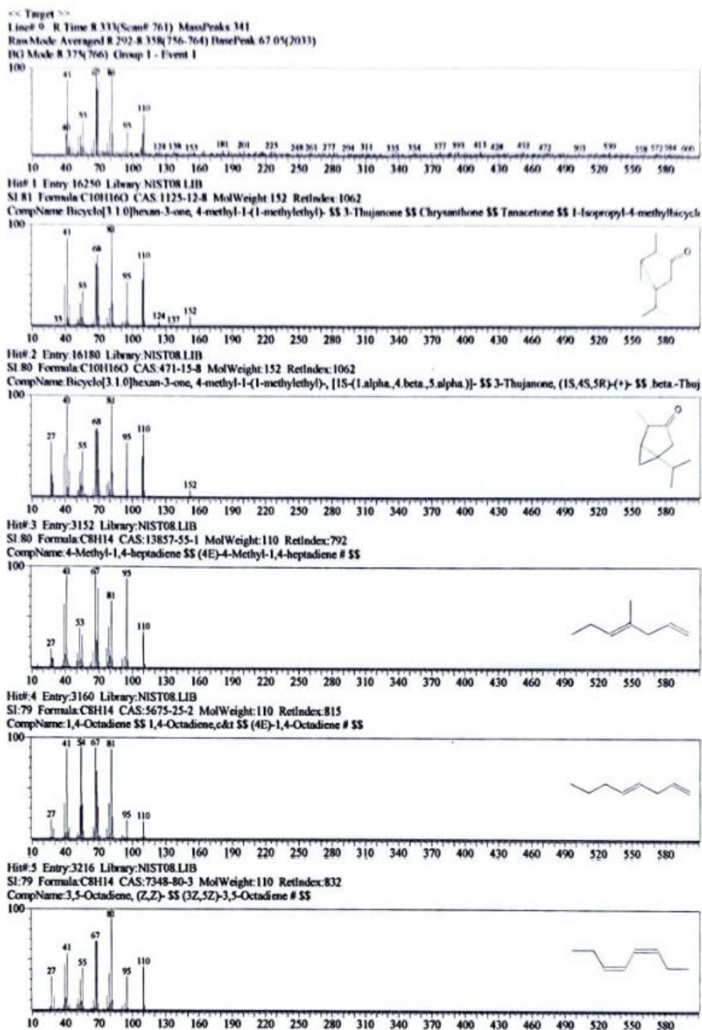
Figure 17. GC-MS mass-spectral library-search output, panel 15 of 27; candidate matches are tentative and not confirmed compound identities.
