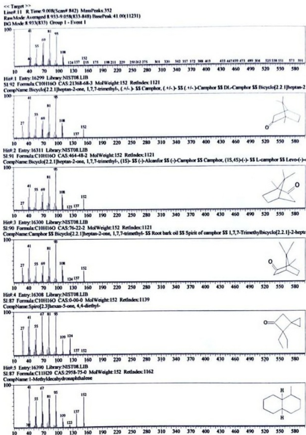
Figure 27. GC-MS mass-spectral library-search output, panel 25 of 27; candidate matches are tentative and not confirmed compound identities.
