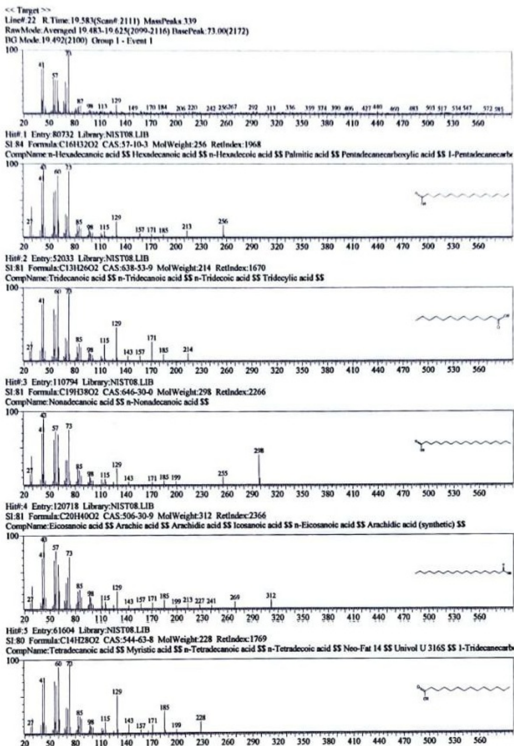
Figure 8. GC-MS mass-spectral library-search output, panel 6 of 27; candidate matches are tentative and not confirmed compound identities.
