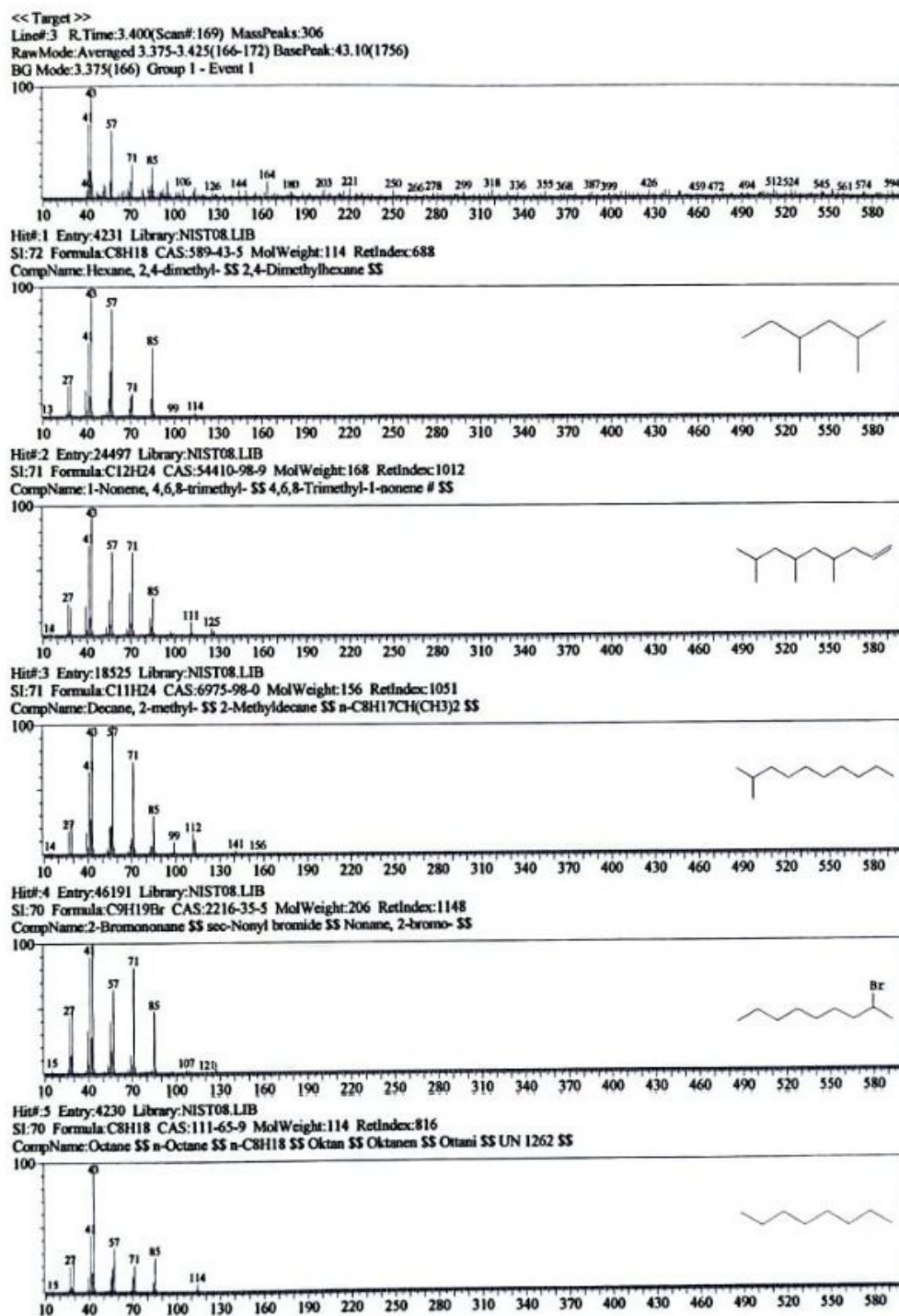
Figure 20. GC-MS mass-spectral library-search output, panel 18 of 27; candidate matches are tentative and not confirmed compound identities.
