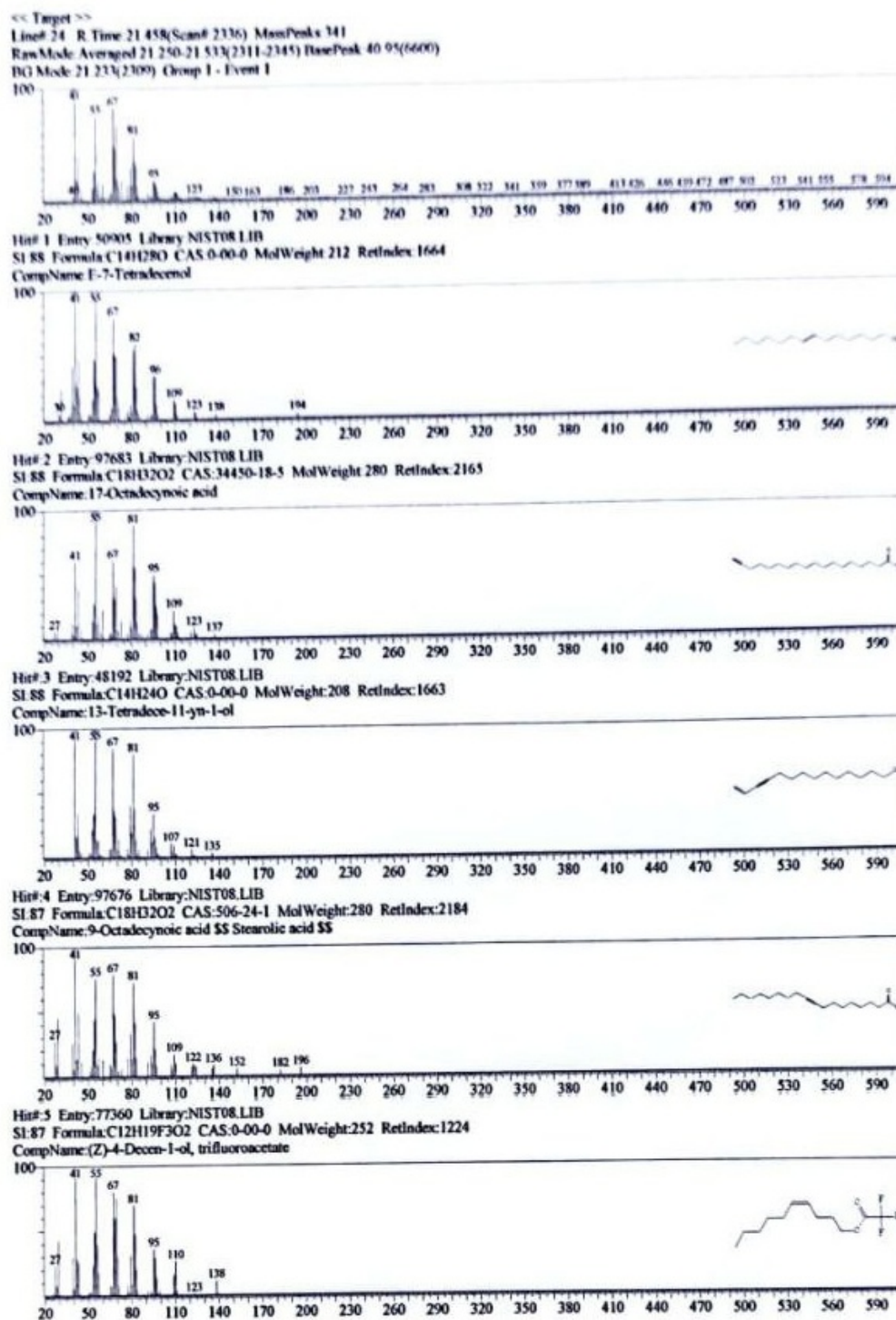
Figure 5. GC-MS mass-spectral library-search output, panel 3 of 27; candidate matches are tentative and not confirmed compound identities.
