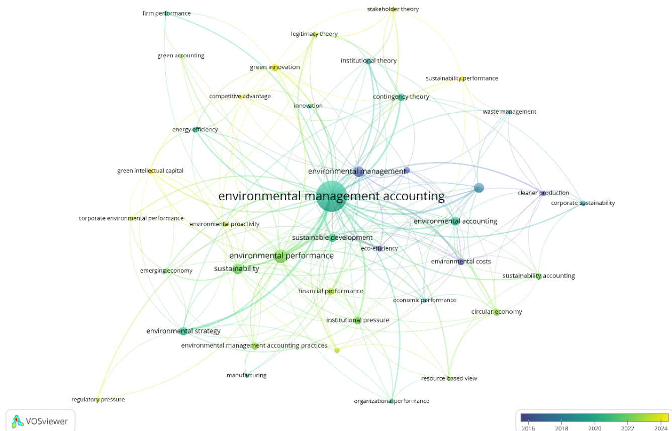
Figure 3. Overlay visualization of author keyword co-occurrence
